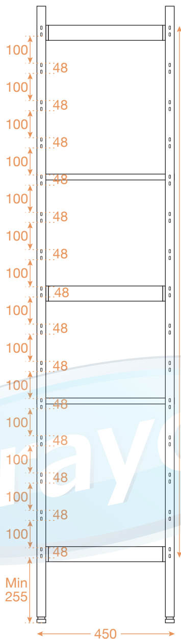
450mm Deep
